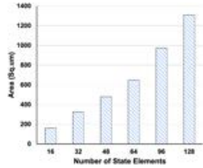
Fig. 8. Impact of increasing the state-elements in the TREE MODE FSM on the Area.
