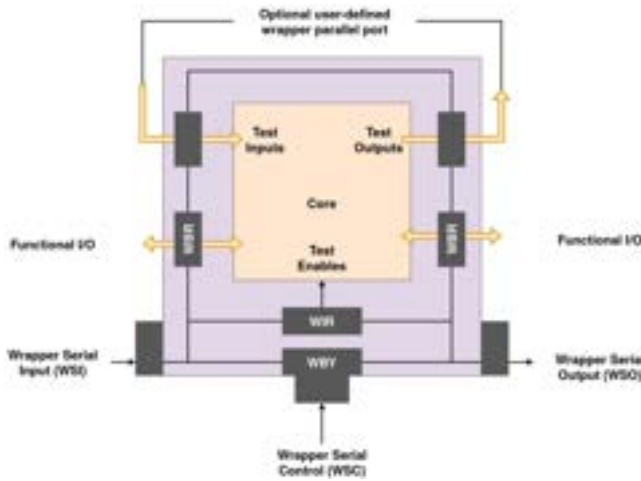
Fig. 3. An example implementation of the IEEE 1500 Core Test Access protocol.
