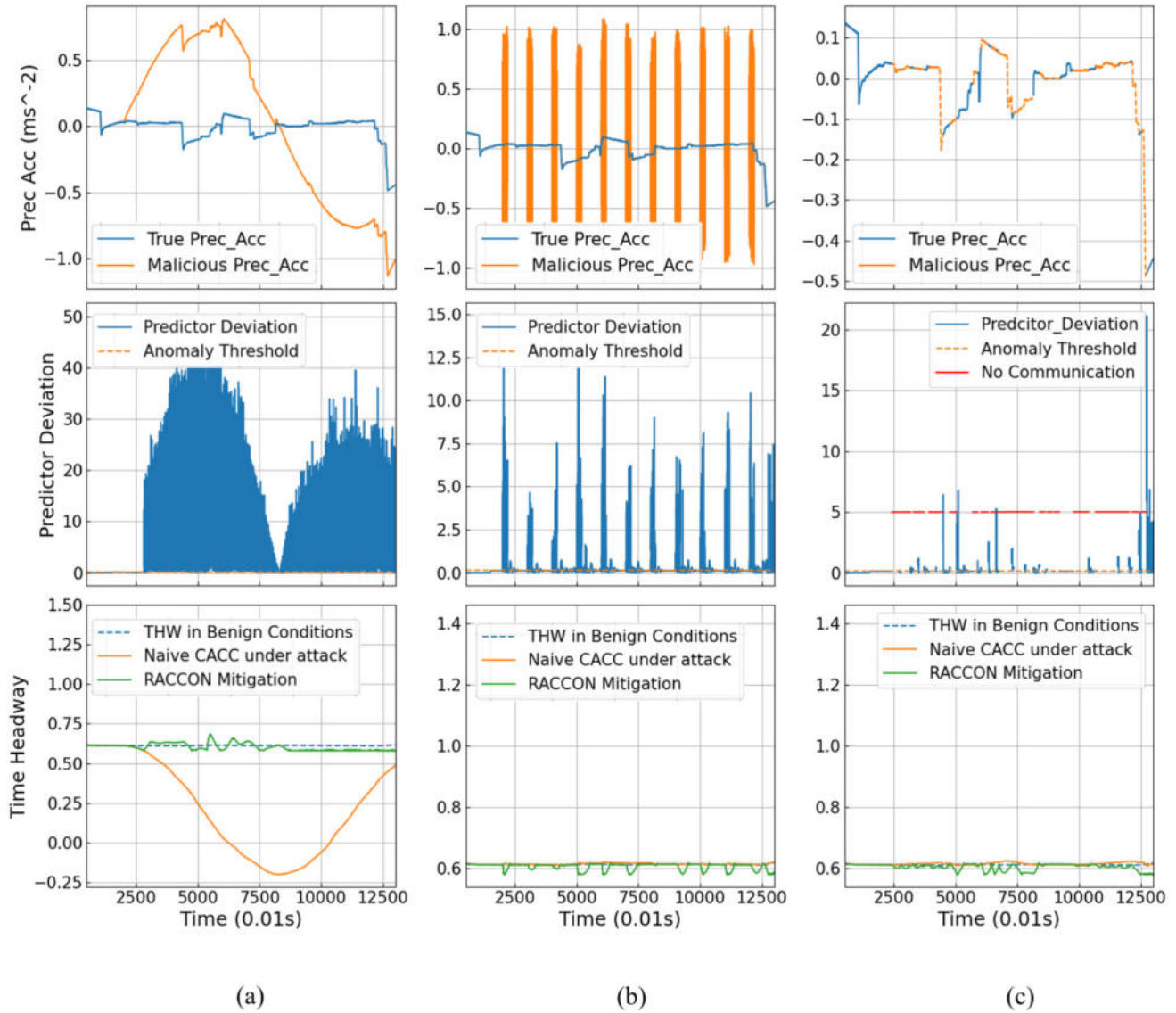
Fig. 14. RACCON Resiliency under Representative N -day Attacks. (a) MITM Attack with continuous sinusoidal bias. (b) Flooding Attack with cluster random bias. (c) DoS Attack with intermittent communication.
