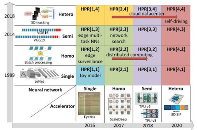
Fig. 3. Neural network-accelerator heterogeneity plane. Blue: early works; green: scaled-up systems; orange: compilers; purple: recent works; red: only AINNS.
