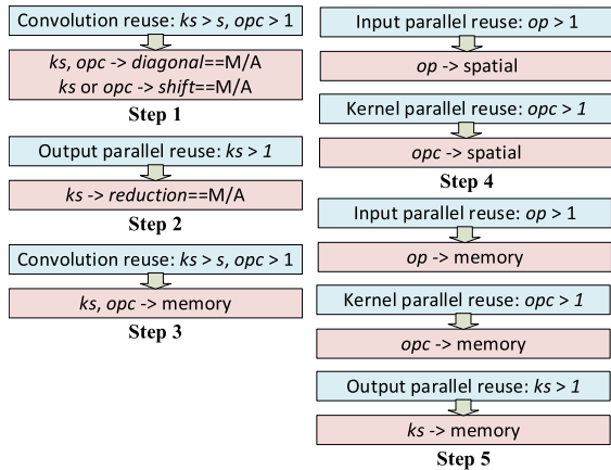
Fig. 10. Local mapping steps. g is unrolled only when there is no other parameter. The algorithm is applicable to both homogeneous and heterogeneous LF-accs.
