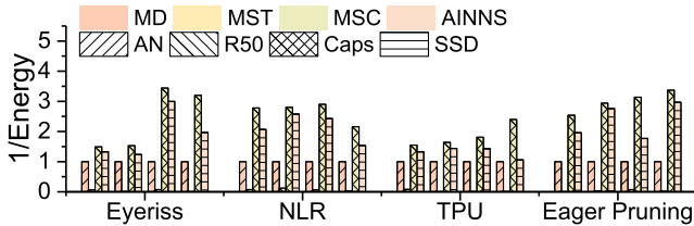
Fig. 12. Data movement energy of single DNNs, normalized to MD.
