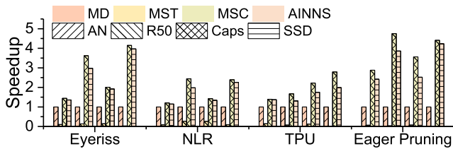
Fig. 11. Speedup of single DNNs, normalized to MD.
