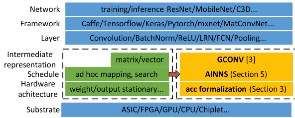
Fig. 1. Neural network acceleration stack before (left) and after (right) our work.
