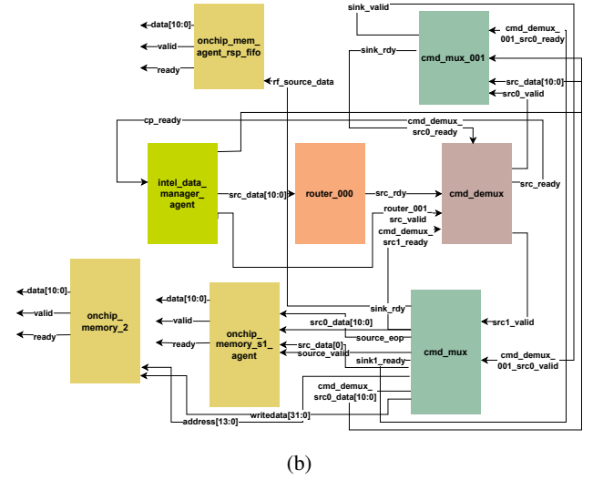
Fig. 3: Analysis of a Single Router Connection inside a NoC fabric (a) Pre-Synthesis (b) Post-Synthesis
