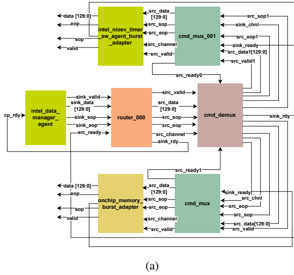
Fig. 3: Analysis of a Single Router Connection inside a NoC fabric (a) Pre-Synthesis (b) Post-Synthesis
