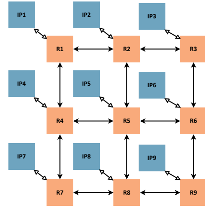
Fig. 1: NoC-based Multi Core Topology
