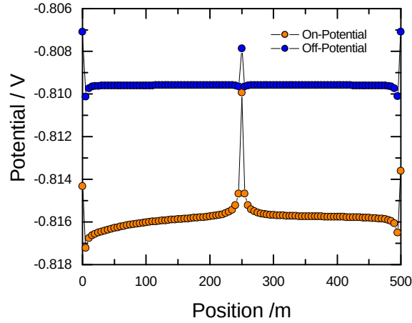
Figure 6-2: On-potential and off-potential on soil surface.
