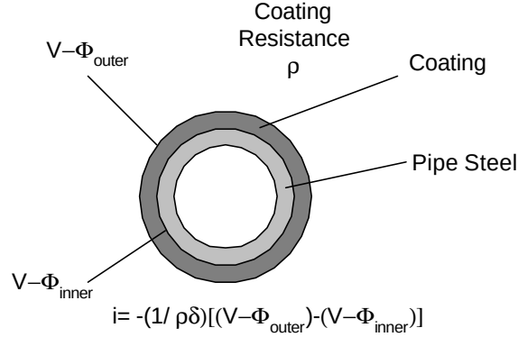
Figure 4-2: Linear relationship between potential drop and current density over the pipe coating.
