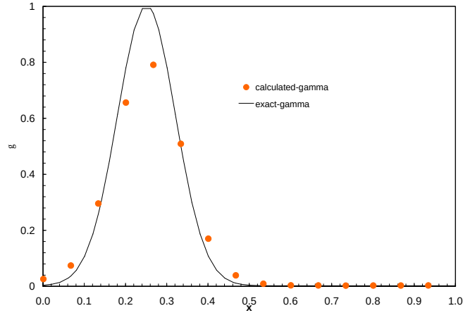
Figure 3-2: Comparisons of the forward and inverse results of TPA method.
