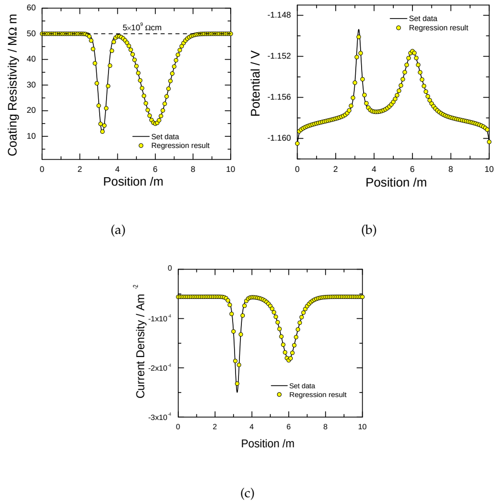
Figure 4-14: Comparison of the set and fitted results for pipe coating with two coating defects: a) coating resistivity; b) potentials; and c) current density.
