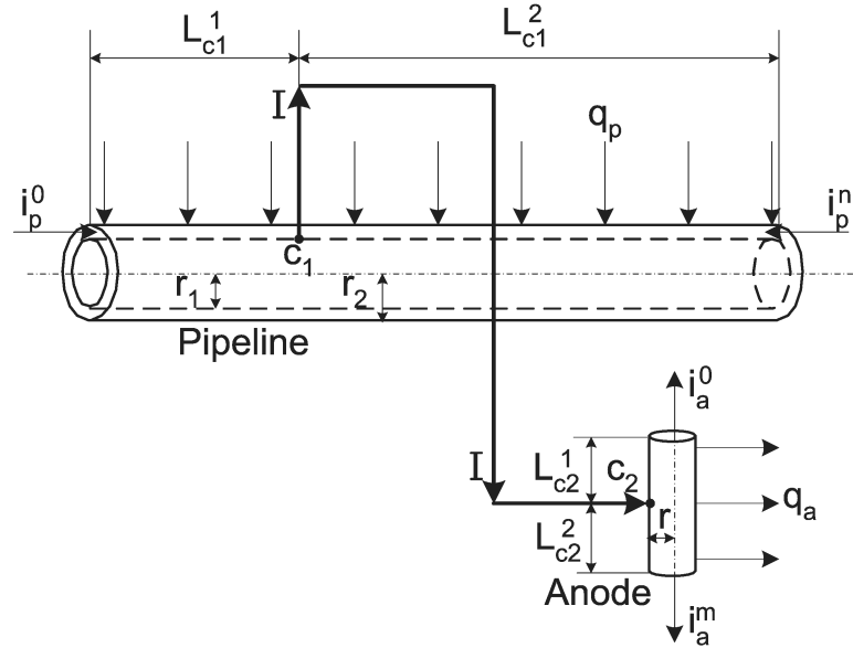
Figure 5-1: Cathodic protection system with variant potential along the pipe and anode.
