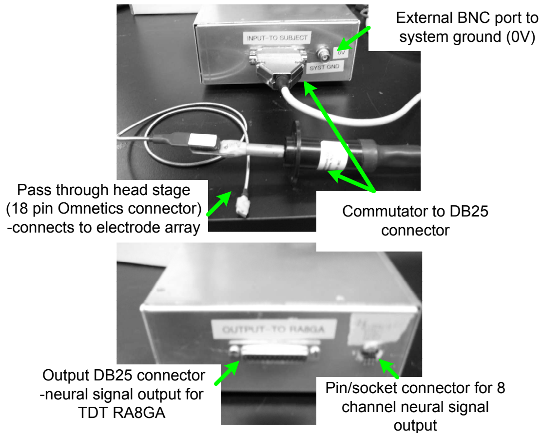
Figure 5-7. Input/output connections for power box.
