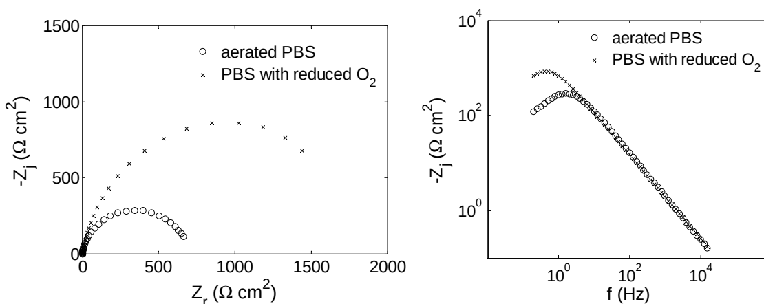
Figure 7-6. Nyquist plot (left) and imaginary impedance as a function of frequency (right) of tungsten electrodes in PBS showing dependence on \text{O}_2 concentration.
