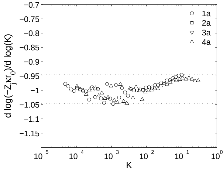
Figure 6-9. Derivative of the logarithm of dimensionless imaginary impedance of the ideal electrodes with respect to \log K . Almost all data points lie within 5% of -1 .
