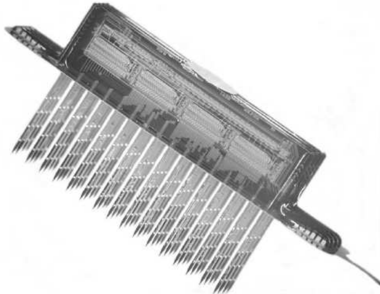
Figure 2-7. 3-D Michigan microelectrode array [reprinted from Proceedings of the IEEE, vol. 96, K. Wise et al., "Microelectrodes, microelectronics, and implantable neural microsystems," p. 1188, Figure 5, 2008, with permission from IEEE].
