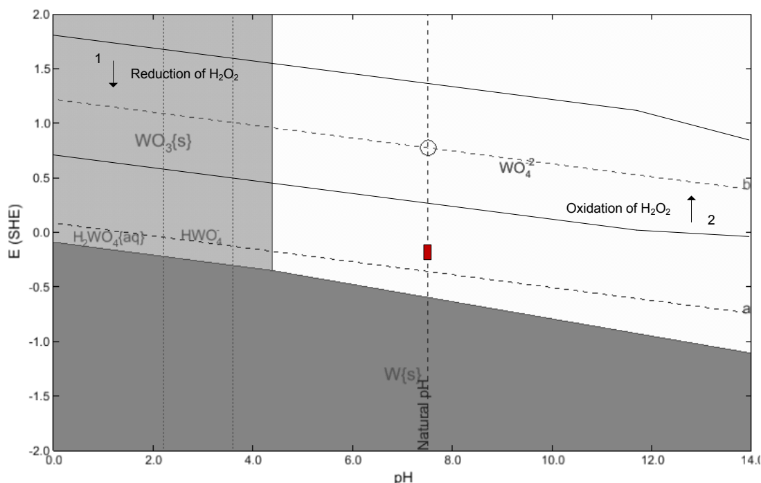
Figure 7-13. Pourbaix diagram of tungsten in an electrolyte containing phosphate buffered saline and 30 mM H_2O_2 . The box shows range of open circuit potential over two days. The diagrams are generated by CorrosionAnalyzer 1.3 Revision 1.3.33 by OLI Systems Inc.
