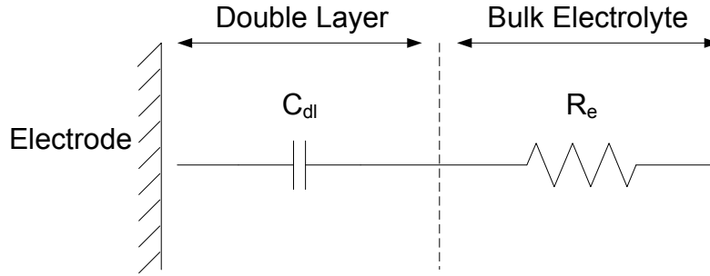
Figure 3-2. Equivalent circuit for the nonfaradaic interface [1].
