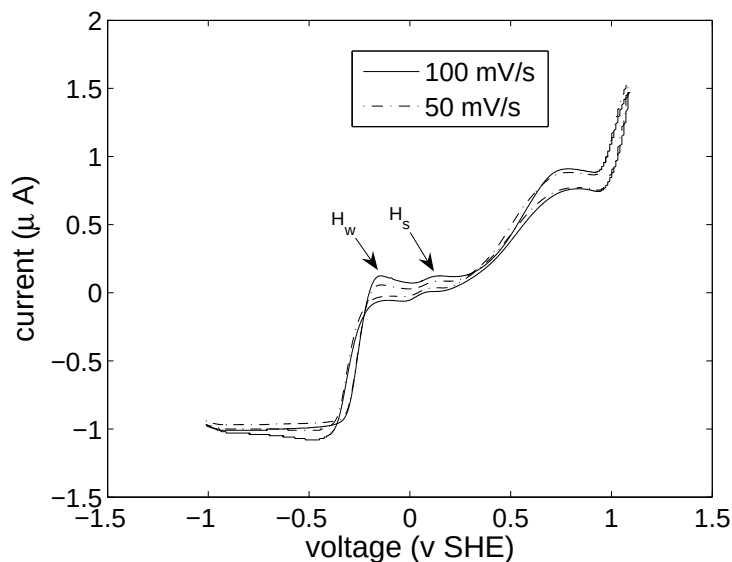
Figure 7-18. Cyclic voltammogram of a platinum electrode in an electrolyte containing PBS and 30 mM \text{H}_2\text{O}_2
