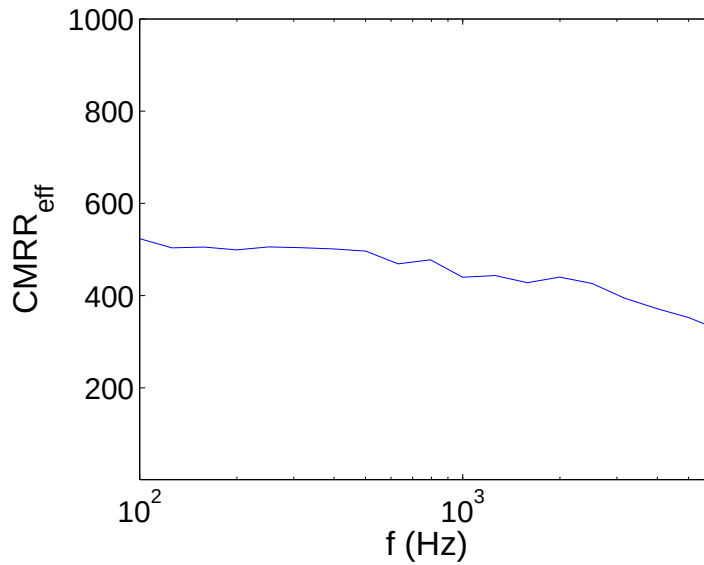
Figure 5-21. Effective common-mode rejection ratio as a function of frequency for impedance values in the UF microelectrode array.
