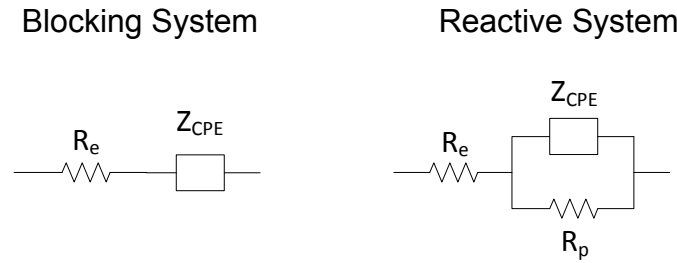
Figure 7-3. Equivalent circuits for blocking and reactive systems [1].
