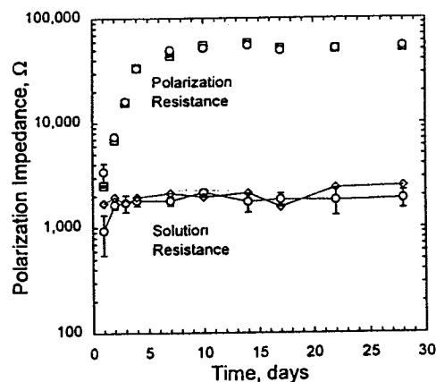
Figure 9. Polarization and solution resistance obtained for a cast iron rotating disk. O) values obtained from measurement model, □) values obtained from a preliminary process model, ◇) independently measured solution resistance.
