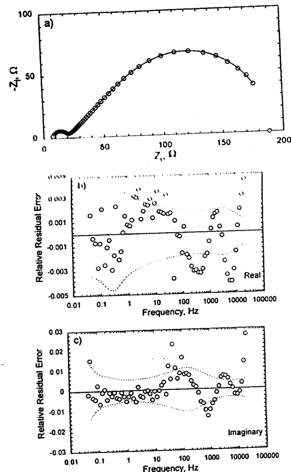
Figure 1. Results of the regression of the process model (equations (2) and (3)) to the data obtained for the reduction of ferricyanide on a Pt disk rotating at 120 rpm and held at \frac{1}{4} of the mass-transfer-limited current. The regression was weighted by the experimentally determined variance, and data shown by the measurement model to be inconsistent were removed from the regressed data set. The frequency range was 0.0461 Hz to 21.4 kHz. a) impedance plane representation where \diamond represents the predicted zero-frequency asymptote, and the line is the regressed fit. b) and c) relative residual error for the regression where the dashed lines represent the bounds for the 95.4% confidence interval for the measurement (i.e., \pm 2\sigma/\hat{Z}' , and \pm 2\sigma/\hat{Z}'' , respectively).
