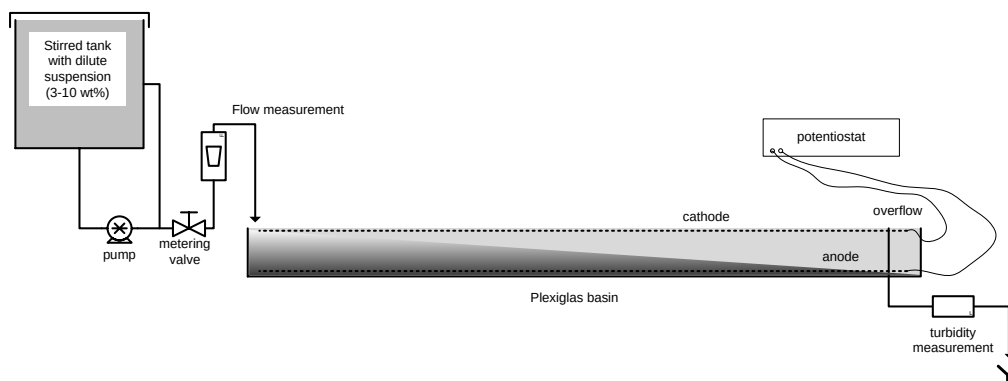
Figure 9-1. Schematic representation of bench-scale settling basin adapted for electrokinetically enhanced separation.
