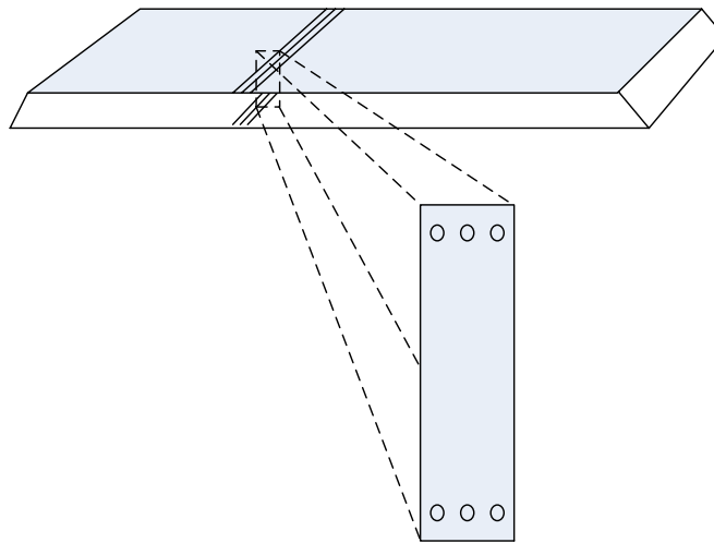
Figure 8-2. Representation of a large clay settling area with one mile long cylindrical electrodes spaced equally along top and bottom surfaces. The zoomed in portion represents a cross-section of the cylindrical electrodes. Although only rows of three cylinders are shown, the simulation was scaled for rows that extend to a distance of one mile.
