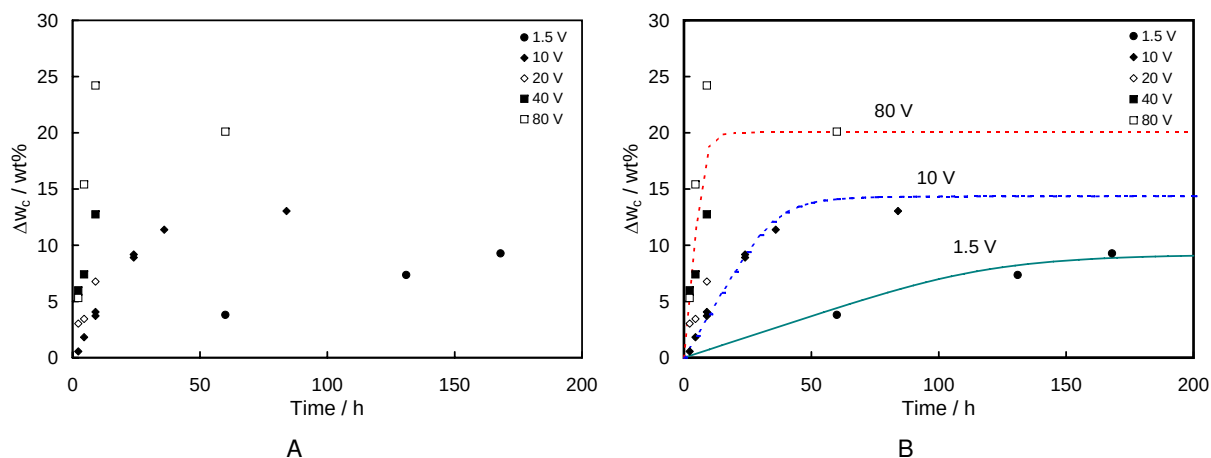
Figure 7-13. Data included in both Figures 7-10 and 7-12 are presented without scaling by the electric field. In B), the constitutive relationship for long times (eq. (7-4)) is fit to the data at three electric field sizes.
