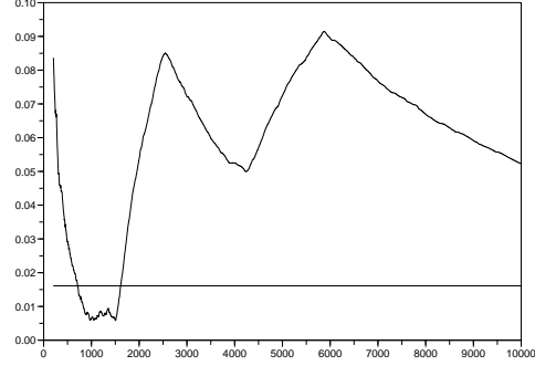
Figure 6: A realization of the sequence of the standard empirical estimates \{\hat{S}_k; 1 \leq k \leq n\} of \mu_1 , for n = 10000 steps of the Gibbs sampler. The horizontal line is the “true” posterior mean of \mu_1 , estimated to be \approx 0.0161 after 15 million Gibbs steps.
