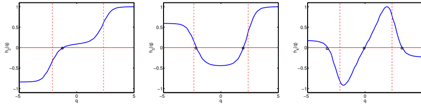
Figure 2. Second to fourth eigenfunction h_2, \dots, h_4 of the generator for the Smoluchowski equation with the perturbed three-well potential and \sigma = 1 . The first eigenfunction h_1 is constant. The dashed lines indicate the main wells of the potential as in Figure 1. Note that the eigenfunctions are remarkable insensitive to large variations of the potential function.
