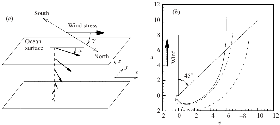
FIGURE 1. (a) Model geometry. (b) Time- and horizontally averaged hodographs of the horizontal current. —, calculations at 90°-latitude; - - -, Ekman profile (1.1); · · · ·, Bessel function solution (3.8) obtained with a piecewise-linear effective viscosity profile (see § 3.3 for details).
