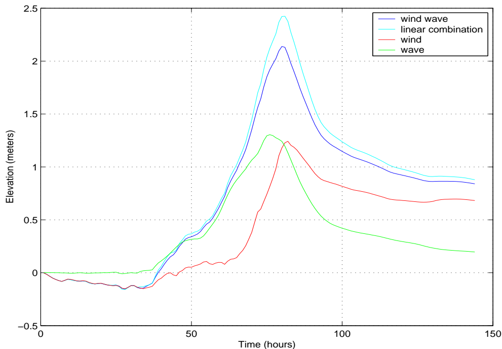
Figure 3-11: The water level at Node-13266:Perdido Bay, FL. We show the surge as predicted by the meteorological forcing, the wave forcing, and the combined forcing. Also plotted is the linear combination of the two individually forced model results.
