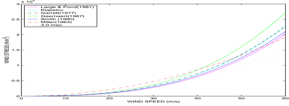
Figure 3-2: Wind stress calculated using the different drag formulas and the cutoff value, plotted vs. wind speed.
