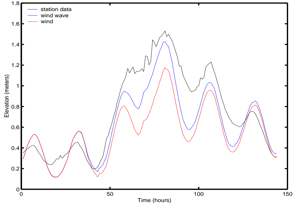
Figure 3–14: Forced by the combination of wave and meteorological inputs, the output from the ADCIRC model at Pensacola Bay is plotted with the historical data recorded by the station at the same corresponding time period. Our prediction is translated in order to more closely match the start time mean water level at the station.
