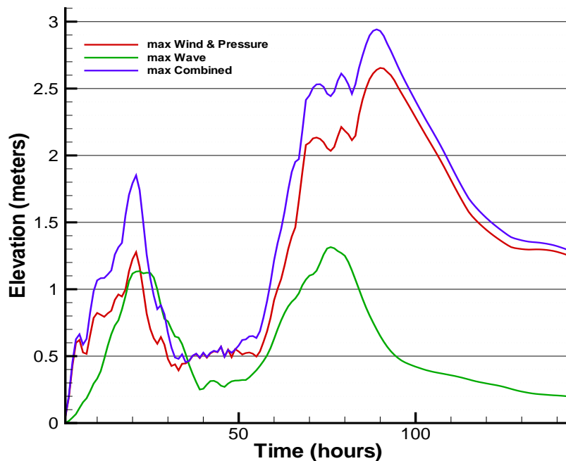
Figure 3–9: For each set of model prediction forcings, the maximum water surface elevation is plotted at every time step.
