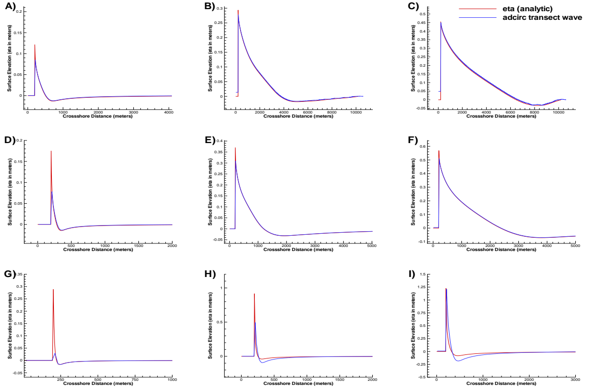
Figure 3-6: Comparison of Model results for wave forcing with the analytic solution for steady state wave set-up. Shown are all nine profile and forcing combinations: A) Shallow profile, weak forcing. B) Shallow profile, medium forcing. C) Shallow profile, strong forcing. D) Mild profile, weak forcing. E) Mild profile, medium forcing. F) Mild profile, strong forcing. G) Steep profile, weak forcing. H) Steep profile, medium forcing. I) Steep profile, strong forcing.
