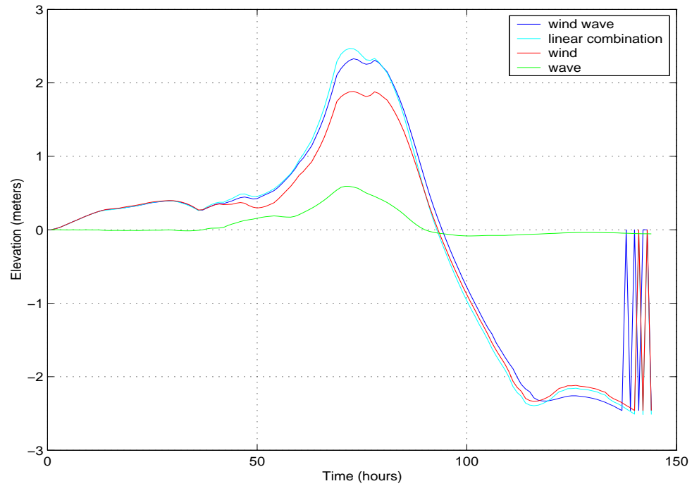
Figure 3-12: The water level at Node-11043: Lake Borgne, LA. We show the surge as predicted by the meteorological forcing, the wave forcing, and the combined forcing. Also plotted is the linear combination of the two individually forced model results.
