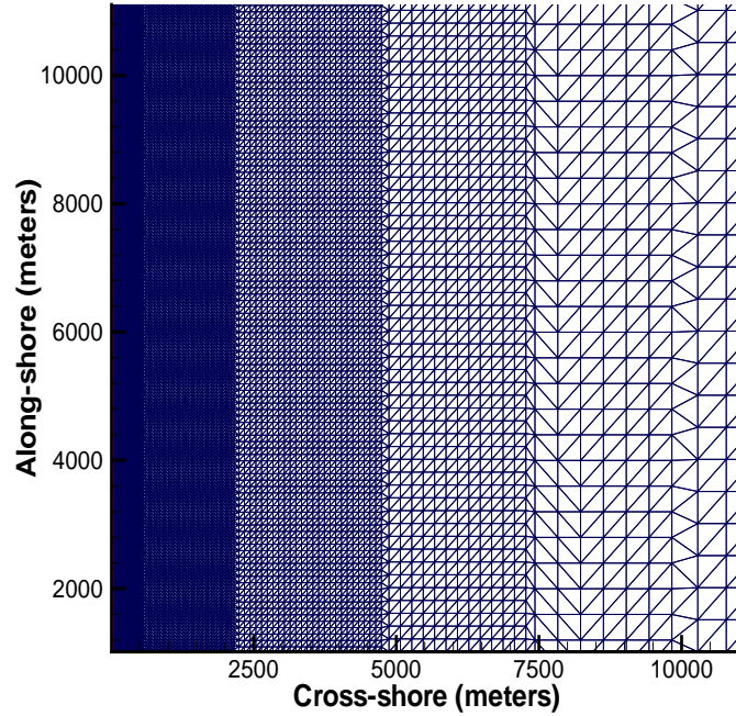
Figure 2-2: Finite Element Grid created with ACE/gredit (resolution at the shoreline is 20 m)
