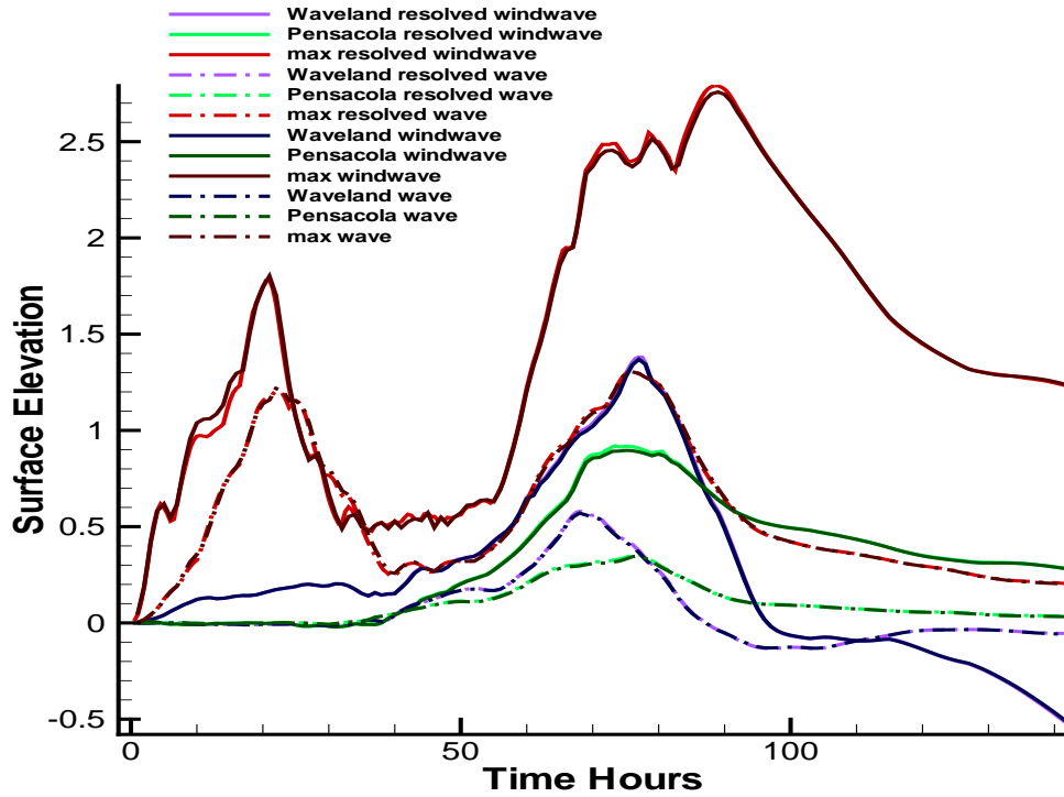
Figure 3–17: We compare the surface response to combined forcing and wave only forcing at the Pensacola location and the Waveland location. Also plotted is the maximum surface elevation over the whole domain for the two forcing combinations. For the resolved case, the finite element grid has 121296 nodes, compared to the 31435 nodes of the current grid.
