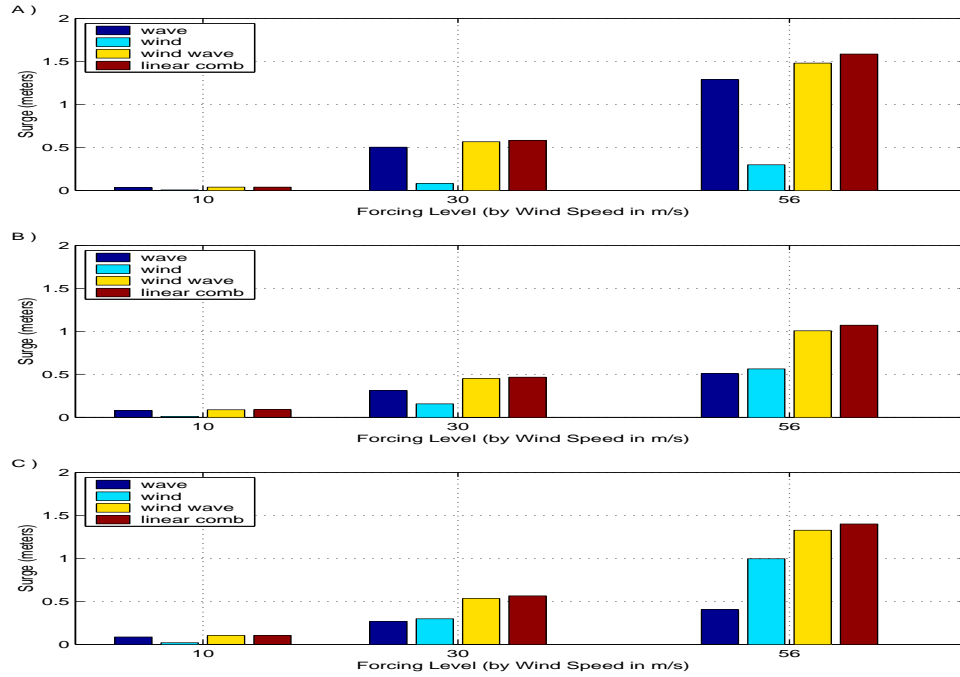
Figure 3–5: The surge levels for each forcing group over each bottom topography (data from Table 3–1) A) Steep slope. B) Mild slope. C) Shallow slope. The wind-wave entry represents the combined forcing for the model run. The linear combination entry represents the sum of the surge predicted from the wind forcing, and that predicted using only the wave forcing.
