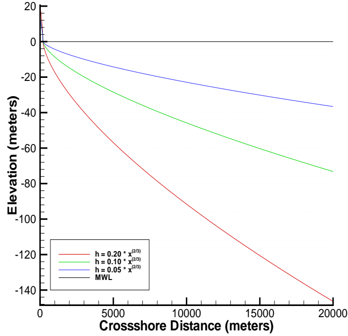
Figure 2–1: Bathymetric contours created to test the wave and wind set-up in the alongshore. We generate a finite element grid, Figure 2–2, for the model domains using ACE/gredit (Turner & Baptista, 1999). Resolution at the shoreline is on the order of 20 meters, and decreases as the depth increases.
