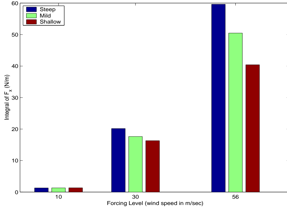
Figure 3–4: The integral sum of \overline{F} output by SWAN for the three different forcings over the three bathymetric profiles. The value of the forcing is given by equation 2–9
