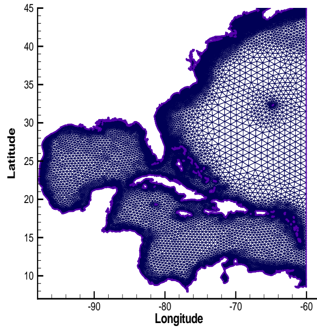
Figure 2–5: Finite Element Grid of the Northwest Atlantic Domain consisting of 31435 Nodes and 58369 Elements. The nodal spacing is 0.03 to 0.06 degree at the coast, 0.016 degree in the inlets, and about 0.5 deg maximum spacing in the Gulf of Mexico.
