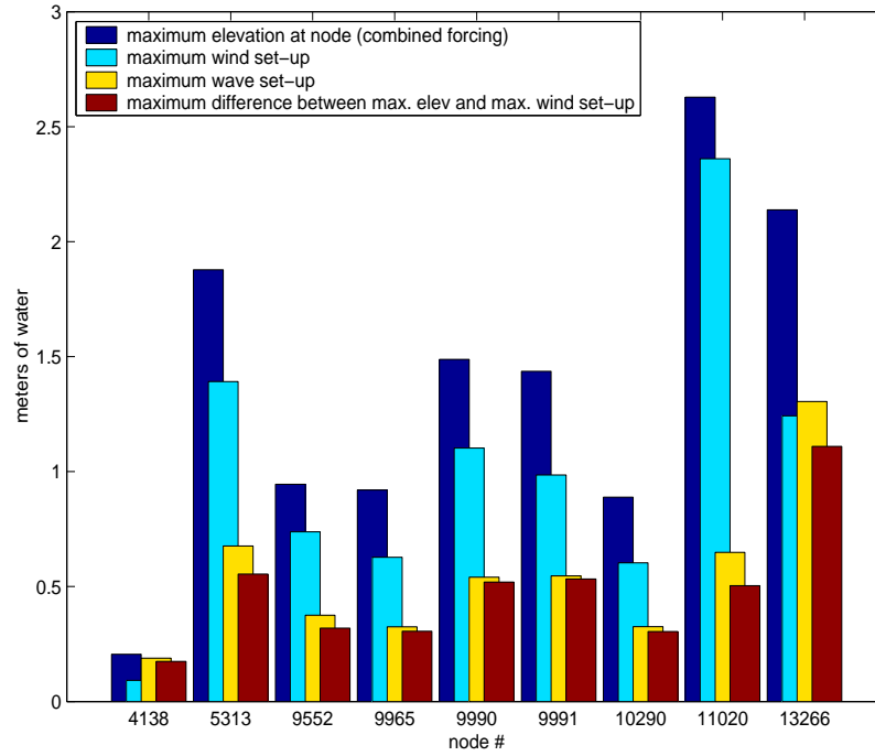
Figure 3–10: For the specified nodes given in Table 3–2, we plot the maximum surge over the duration of the simulation for combination of each forcing. Also plotted is the maximum difference between the combined forcing and wind only forced elevation.
