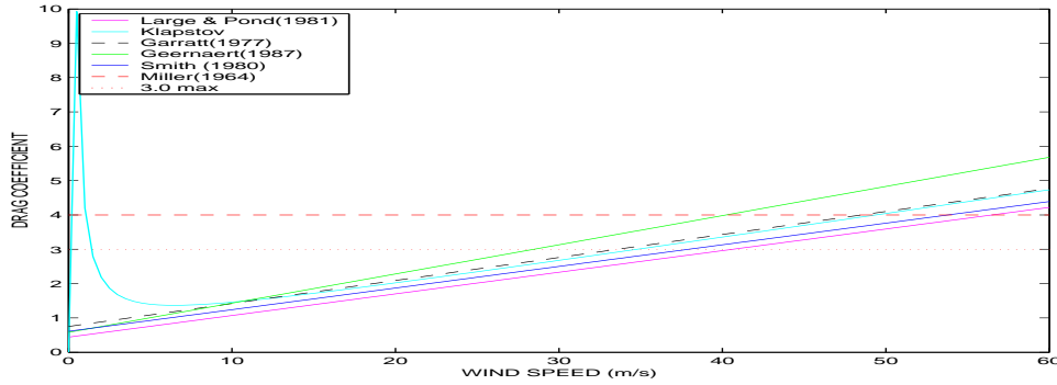
Figure 3-1: The seven drag coefficient formulations plotted vs. wind speed.
