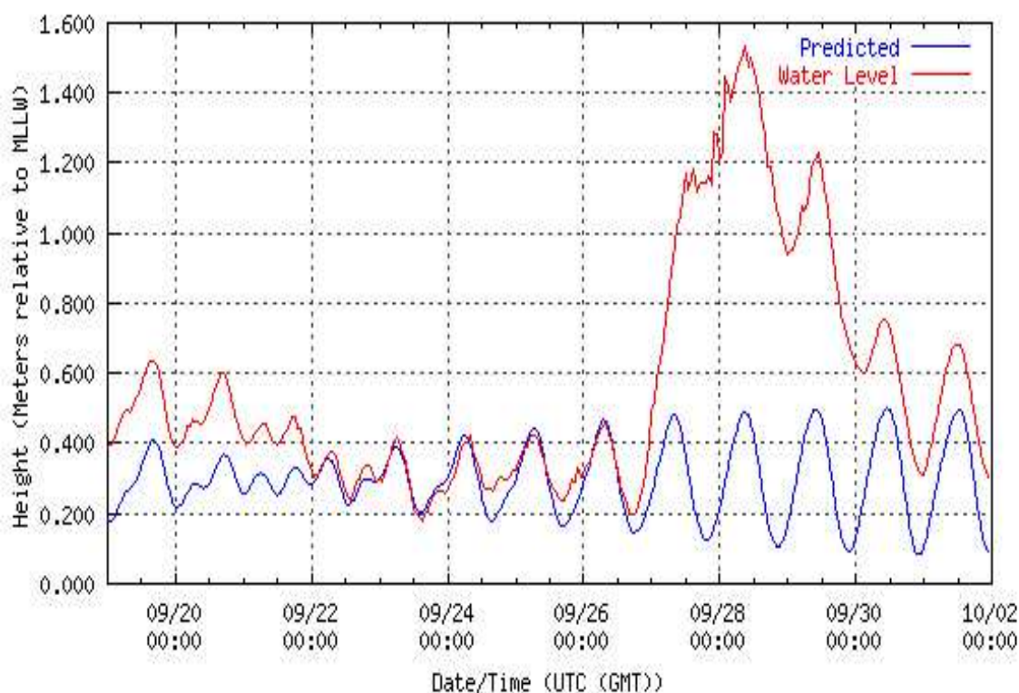
Figure 3–13: The NOAA station data for Pensacola Bay, FL. Water elevation is referenced to MLLW.
