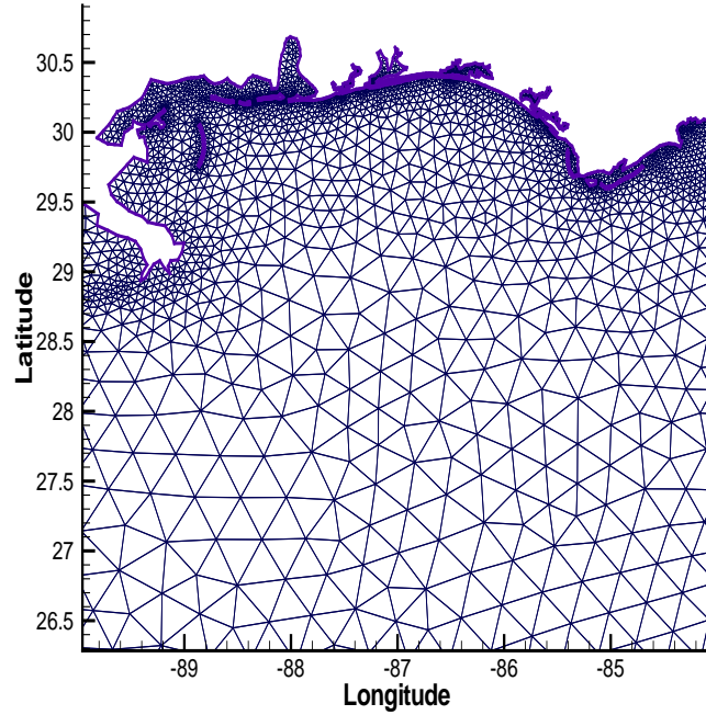
Figure 2–6: The Gulf Coast region of our model domain (Louisiana to Florida). This is where hurricane Georges made landfall in the Continental U.S.
