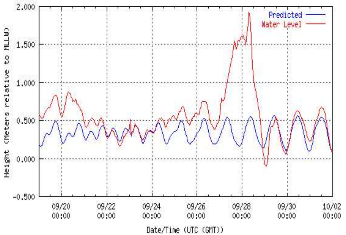
Figure 3-15: The NOAA station data for Waveland, MS (water elevation is referenced to MLLW).
