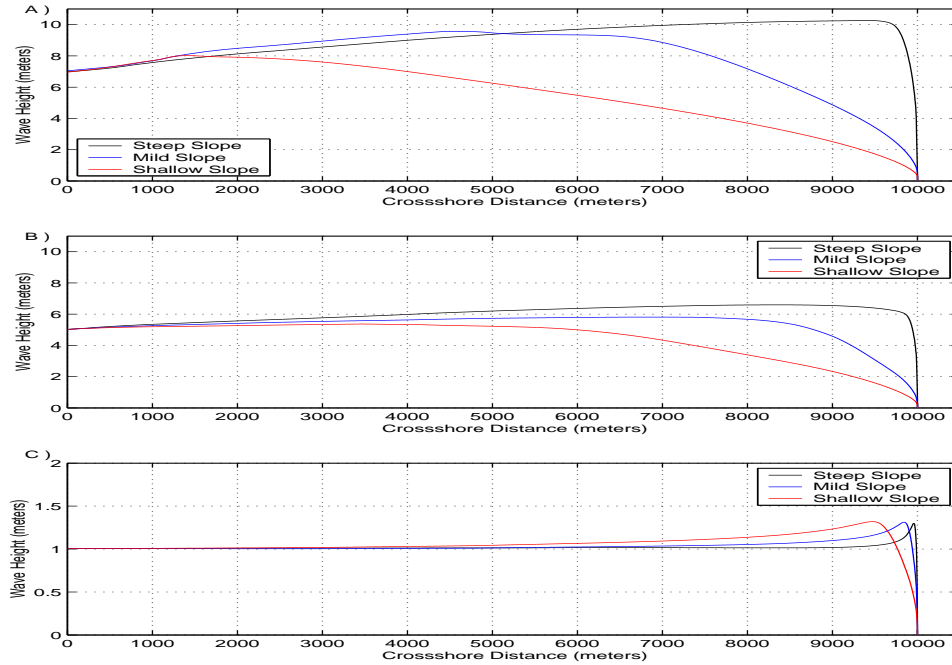
Figure 2-3: The wave fields output by SWAN over the three bathymetric contours. A) Strong forcing. B) Medium forcing. C) Weak forcing.
