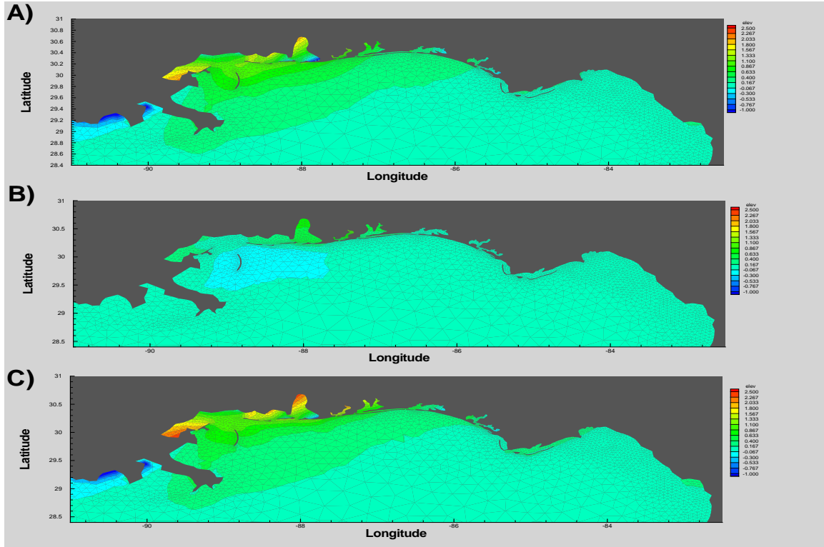
Figure 3–8: A series of surface contour plots shows the surge as hurricane Georges make landfall, t=82 h. A) Surface elevation generated from the meteorological forcing. B) Surge created by wave forcing. C) Surge generated from the combined forcing.
