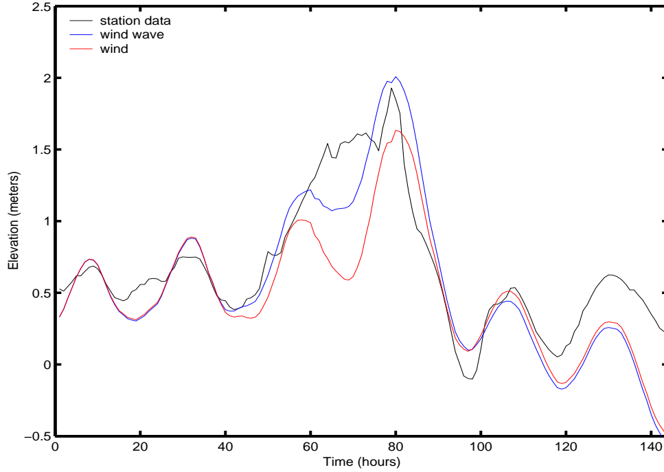
Figure 3–16: Forced by the combination of wave and meteorological inputs, the output from the ADCIRC model at Waveland is plotted with the historical data recorded by the station at the same corresponding time period. Our prediction is translated in order to more closely match the start time mean water level at the station.
