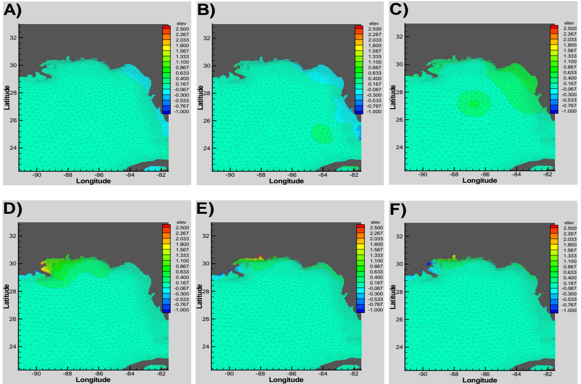
Figure 3–7: A series of surface contour plots shows the surge as hurricane Georges makes its way across the Gulf of Mexico and makes landfall (prediction was made with the combined forcings). A) t = 10 hours into the simulation. B) t = 30 hours. C) t = 50 hours. D) t = 70 hours. E) t = 90 hours. F) t = 110 hours.
