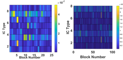
Fig. 8. Block-wise Intra-chip Distance Variability.
