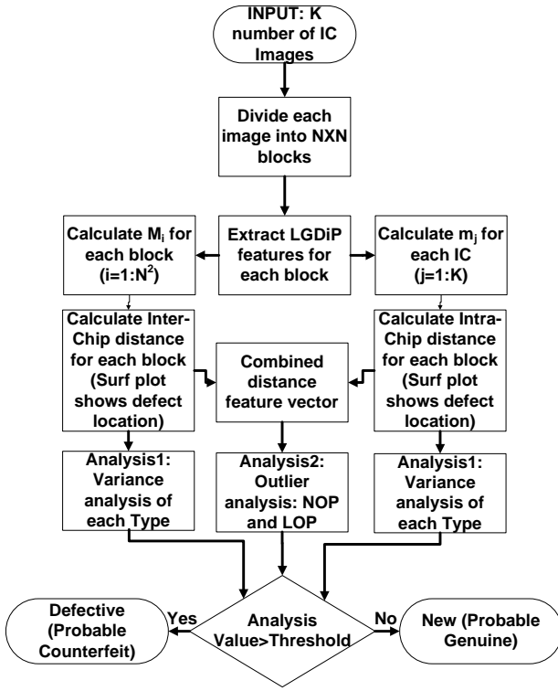
Fig. 3. Flowchart of defect detection methodology.
