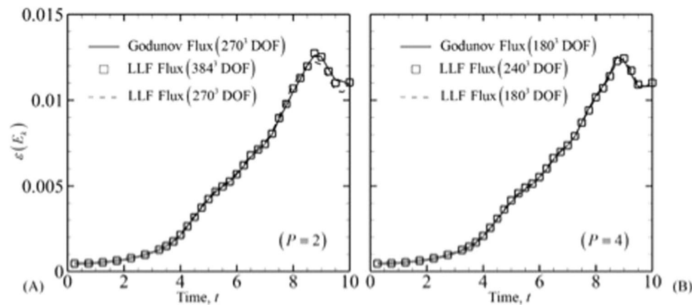
Figure 3. Comparison of energy dissipation rate for different inviscid numerical fluxes at different degrees of freedom and polynomial order. Dissipation rate for (A) P=2 and (B) P=4 .
