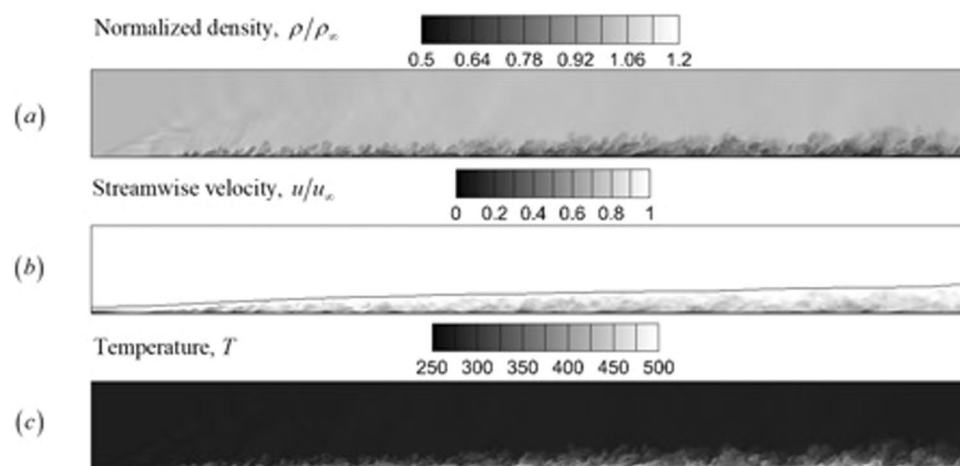
Figure 14. Instantaneous contours for the turbulent boundary layer at M=2.25 . (a) Normalized density field, (b) normalized instantaneous velocity, and (c) temperature (K) are plotted.
