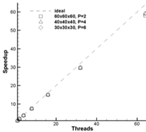
Figure 12. Parallel scaling of MIG code via OpenMP.
