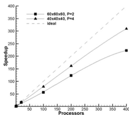
Figure 11. Parallel scaling of MIG code via MPI.
