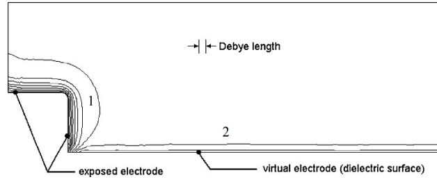
Figure 7. Collective wall effects of the exposed powered electrode and virtual electrode (dielectric region). 1- Anode Sheath, 2- Cathode Sheath. 3
